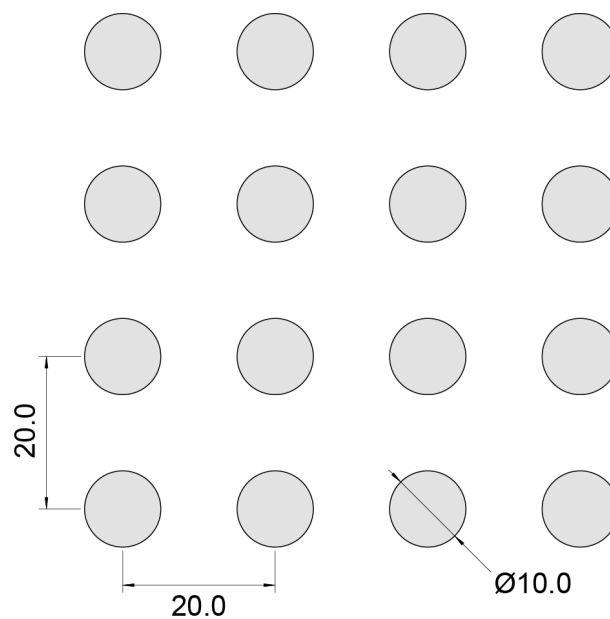
Diameter 10mm Open Area 19.6%
